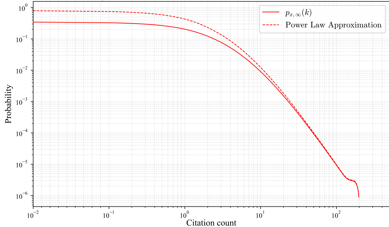
Type A: p_{x,\infty}(k) vs Power Law for Citation Distribution in 28,005 Network
